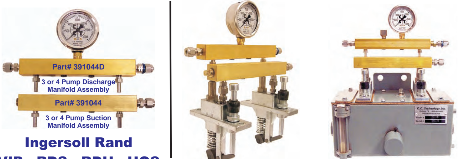
3 & 4 Pump Suction & Discharge Assembly (Shown on IR-HOS Lube Box)
