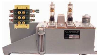
AJAX Special: 1 Pump for Engine - 1 Pump for Compressor
